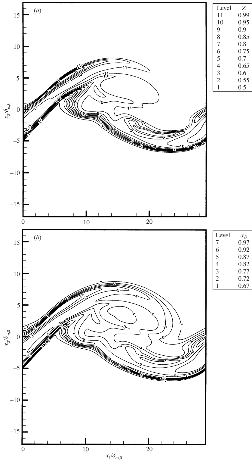
FIGURE 9 (corrected). The compression factor (a) and the mass diffusion factor (b) in the braid plane at the non-dimensional time t\Delta U_0/\delta_{\omega,0} = 100 .
